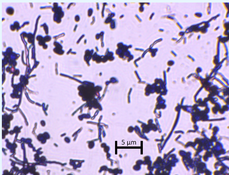
Gram stain of fermentation liquid from crock ferment (100X Mag)
